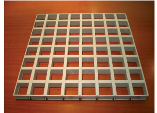
595x595mm lay on open cell ceiling tile with 4 sides trimming (put on tee grids directly) optional spec.:50x50mm/75x75mm/100x100mm/120x120mm/150x150mm/200x200mm
